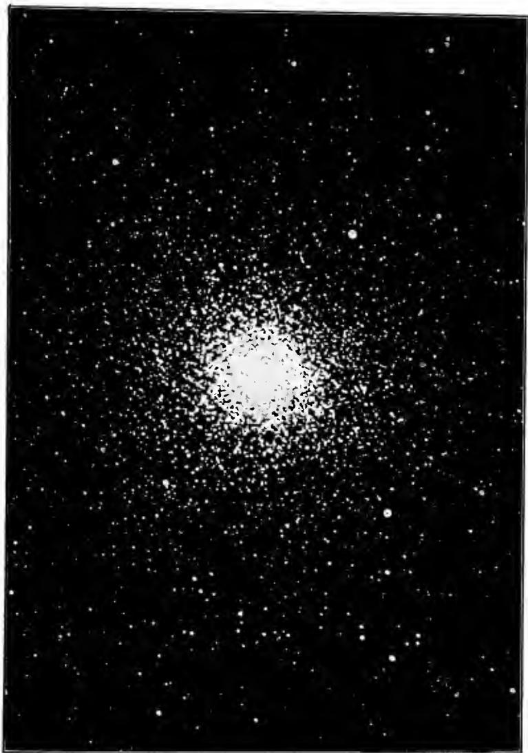
GREAT SOUTHERN STAR-CLUSTER, OMEGA CENTAURI
